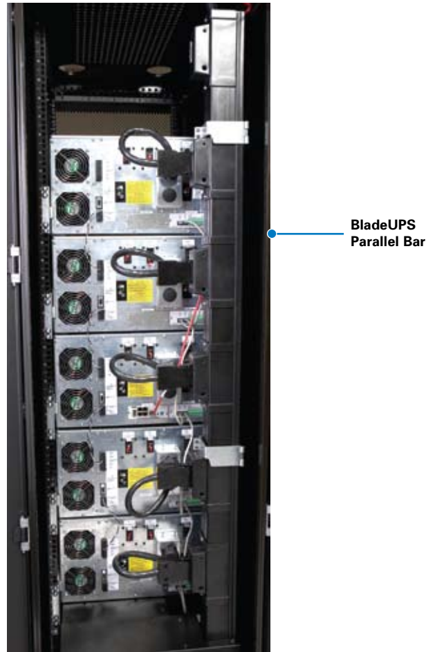
The BladeUPS Parallel Bar easily connects up to six modules in parallel.
